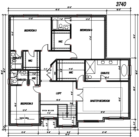
Second Floor Plan 2155 sq. ft. (Includes open area)
